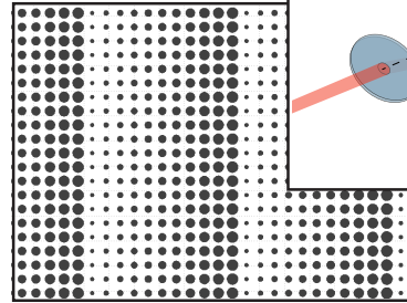
Beam Diffraction/Steering (Flat Blazed Gratings)
